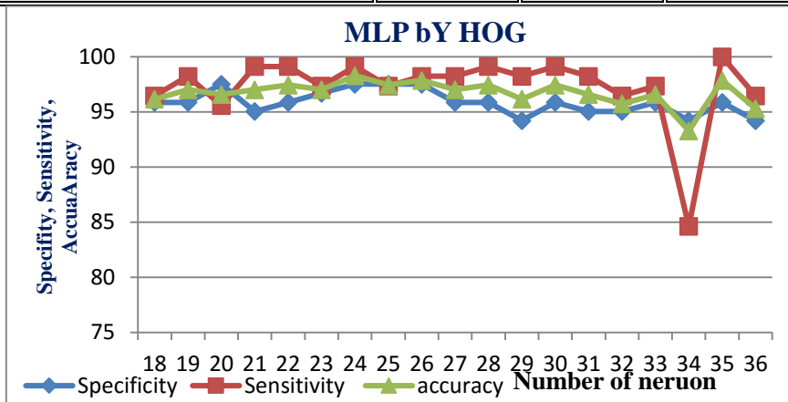
Figure 11: Graph is illustrating that the Number of neuron in hidden layer =24 which considered the best results (specificity=97.52, sensitivity=99.12 and accuracy =98.29) in MLP by using HOG
