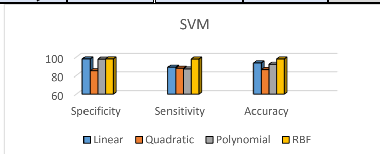
Figure 9: Graph is illustrating that SVM using LBP by different kernel function with test dataset.
