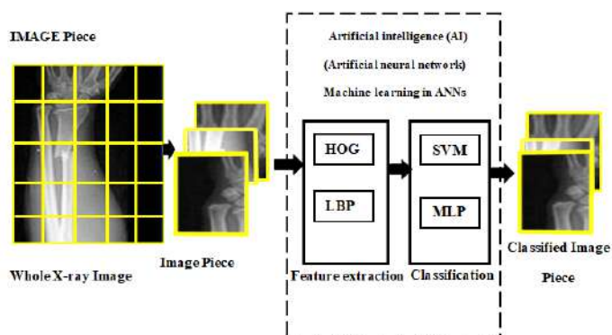
Figure 3: The long bone fracture detection System Overview
