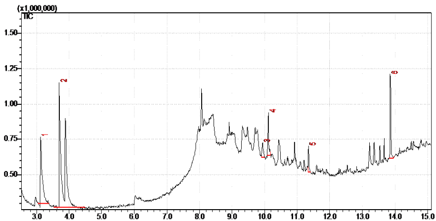
Figure 4: LC-MS profile of S. incanum fruit extract, E3.
